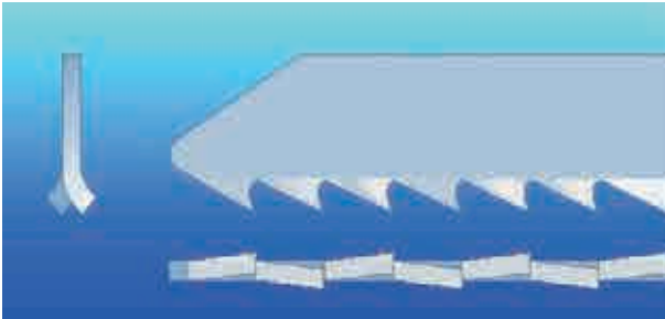
Milled and side set teeth
